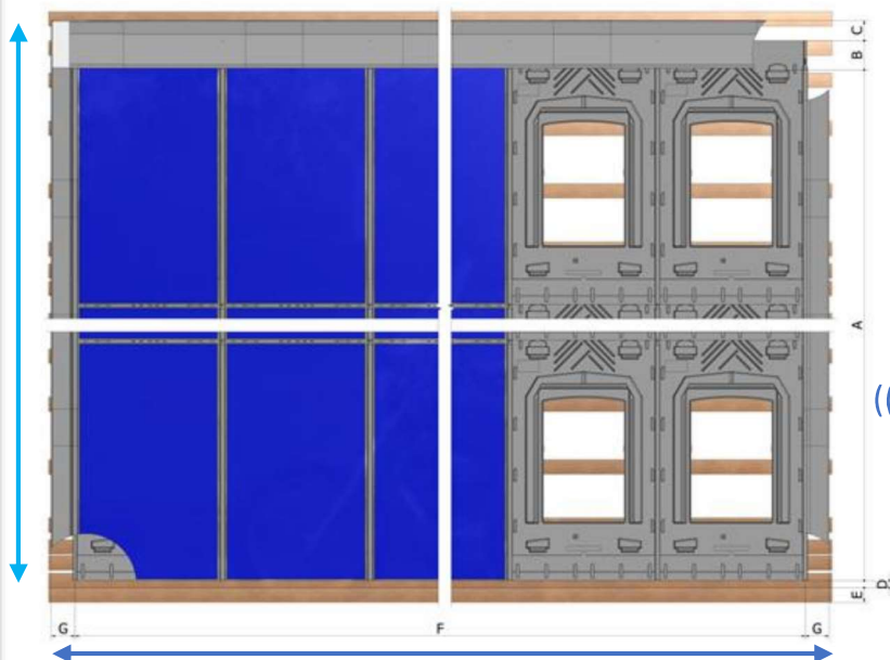
Plaques GSE - PORTRAIT
