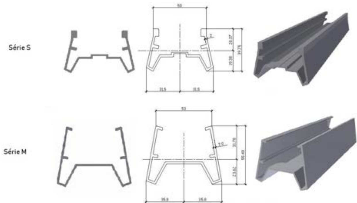
Figure 10 – Éclisses
