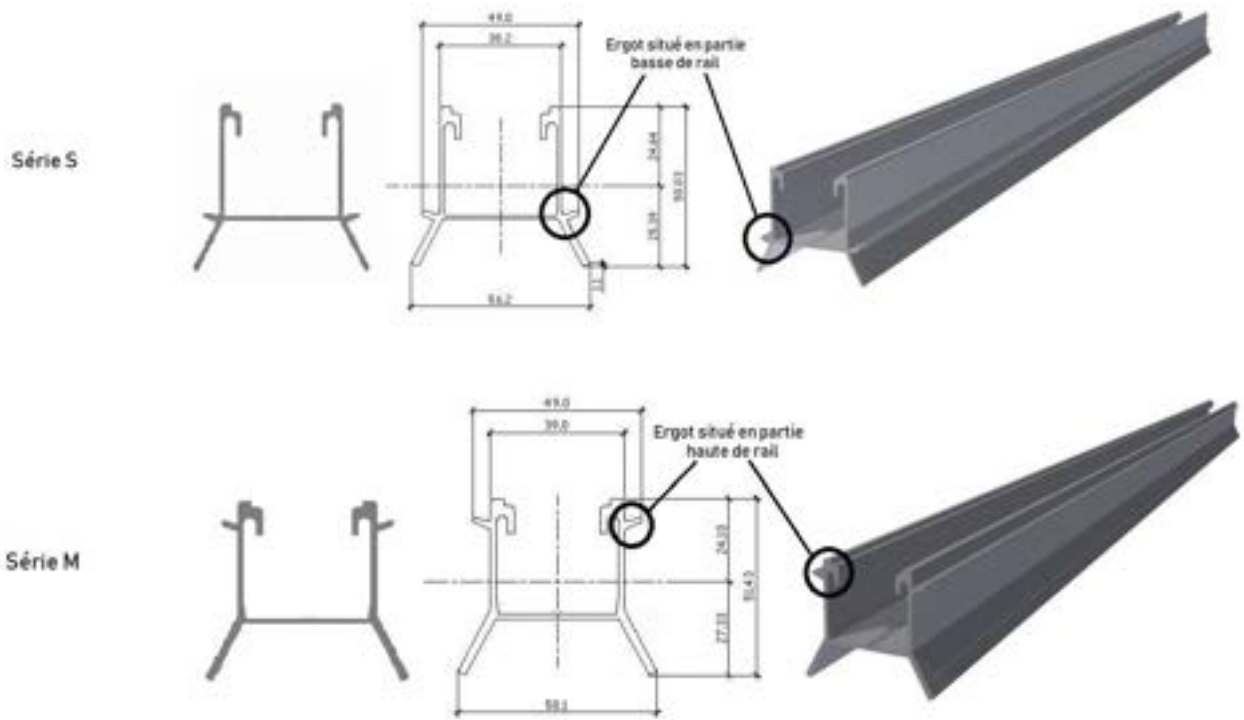
Figure 9 – Rails
