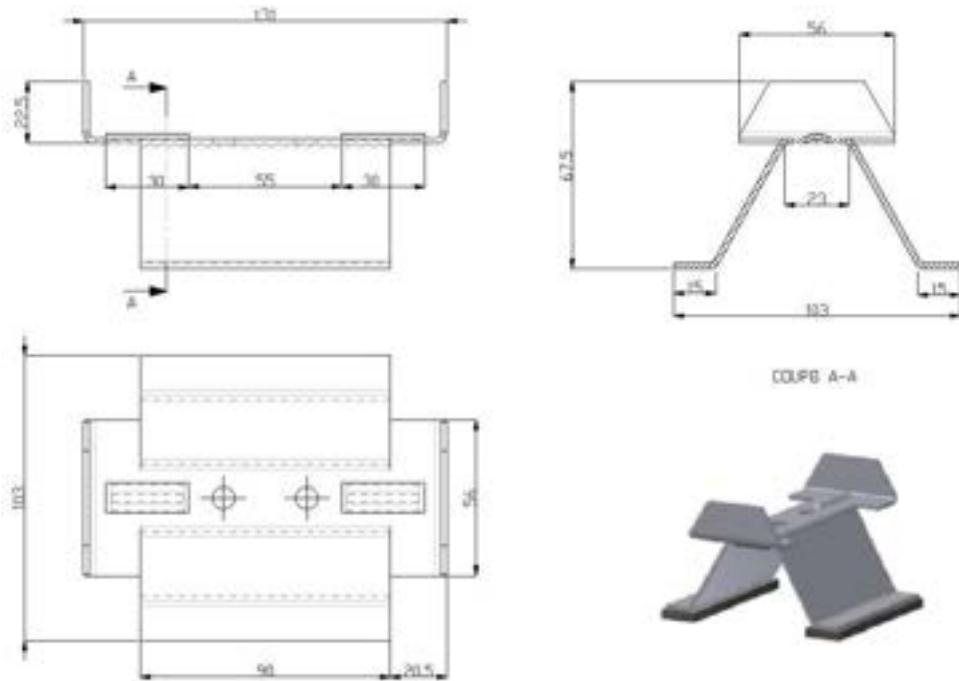
Figure 4 – Rehausse inférieure (Brevet FR1005097)
