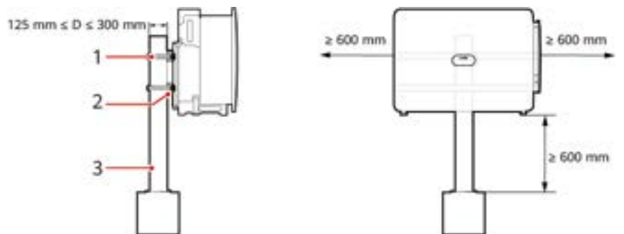
Figure 4-17 Installation de la pince de fixation
