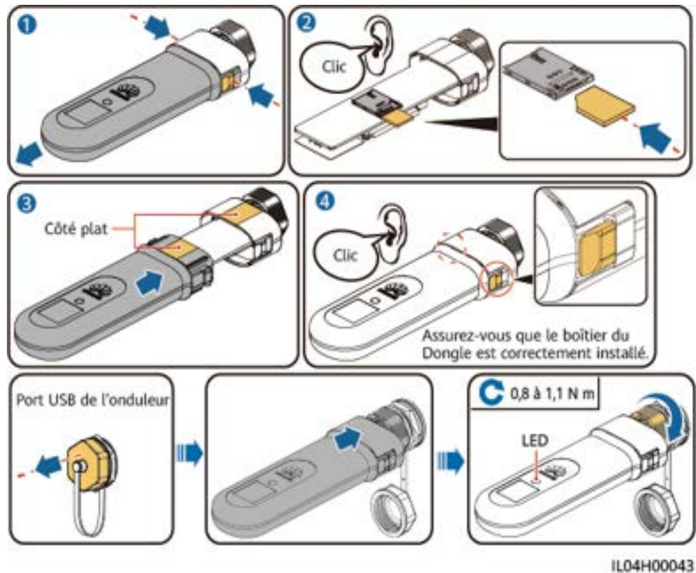
Figure 5-20 Installation du Smart Dongle 4G (SDongleB-06)
