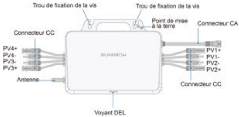
Figure 3-6 Conception externe
