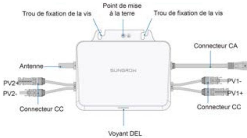
Figure 3-4 Conception externe
