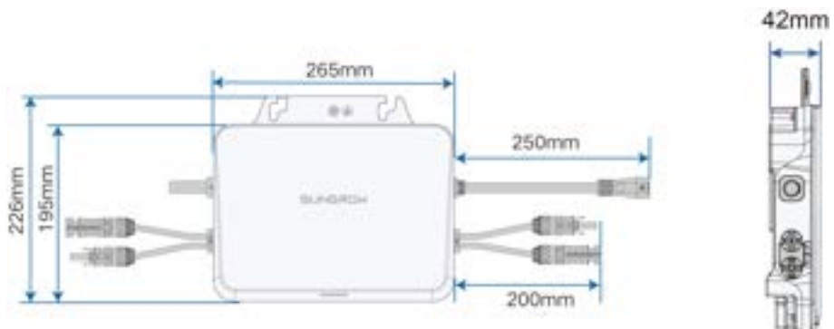
Figure 3-5 Dimensions
