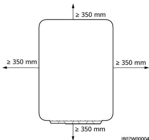
Figure 4-2 Distances
